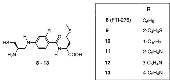
Figure 3. Peptidomimetics with aromatic substitution at the 2-position of 4-aminobenzoic acid.
