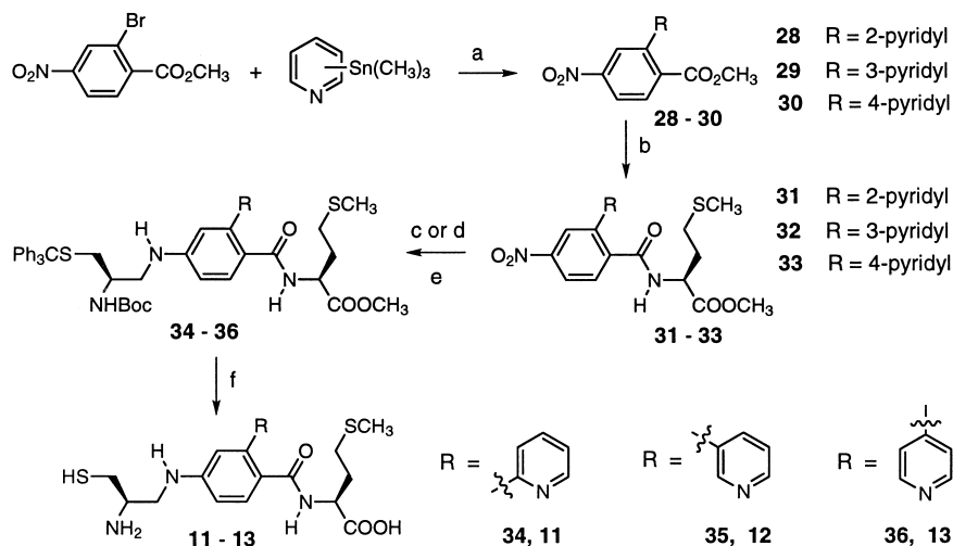
Scheme 4. Preparation of pyridine containing peptidomimetics 11–13 . Reagents; (a) \text{Pd(PPh}_3)_2\text{Cl}_2 , \text{CuI} , \text{LiCl} , toluene; (b) (1) aqueous \text{LiOH} , methanol, (2) (L)-methionine methyl ester, EDCI, HOBT; (c) \text{SnCl}_2 hydrate; (d) Raney Ni, hydrazine, methanol; (e) N -Boc-S-trityl-(L)-cysteinyl, \text{NaB(CN)H}_3 , methanol; (f) (1) aqueous \text{LiOH} , THF, (2) TFA, \text{Et}_3\text{SiH} .
