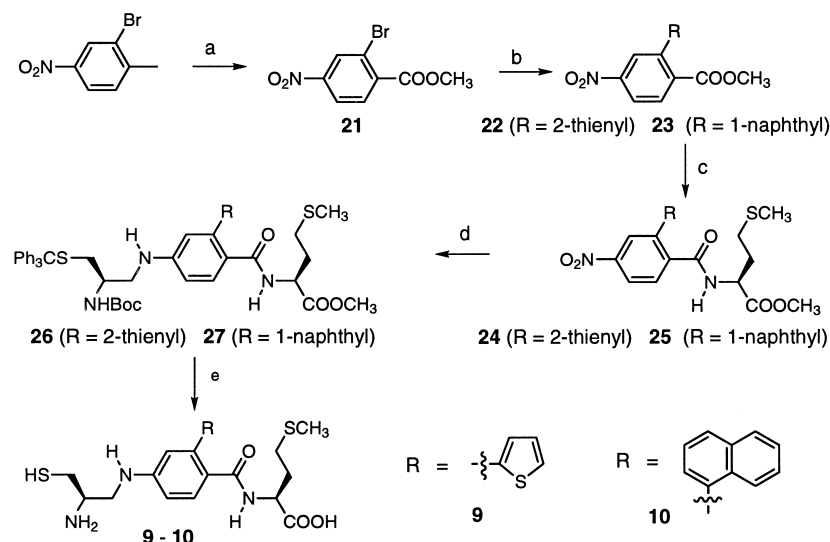
Scheme 3. Preparation of peptidomimetic 9 and 10 . Reagents: (a) (1) \text{KMnO}_4 , aqueous pyridine, (2) methanol, \text{SOCl}_2 ; (b) (1) 2-thienylboric acid or 1-naphthylboric acid, \text{Pd(PPh}_3)_4 , DMF; (c) (1) aqueous \text{LiOH} , MeOH, THF, (2) (L)-methionine methyl ester, EDCI, HOBT; (d) (1) \text{SnCl}_2 hydrate, (2) N -Boc-S-trityl-(L)-cysteinyl, \text{NaB(CN)H}_3 , methanol; (e) (1) aqueous \text{LiOH} , THF, (2) TFA, \text{Et}_3\text{SiH} .
