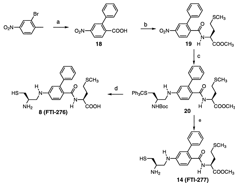
Scheme 2. Synthesis of peptidomimetic FTI-276 and FTI-277. Reagents: (a) (1) phenylboric acid, Pd(OAc) 2 , aqueous acetone, (2) KMnO 4 , aqueous pyridine; (b) (1)-methionine methyl ester, EDCI, HOBT; (c) (1) SnCl 2 hydrate, (2) N -Boc-S-trityl-(L)-cysteinal NaB(CN)H 3 ; (d) (1) LiOH, THF, (2) TFA, Et 3 SiH; (e) (1) HgCl 2 , methanol, (2) H 2 S, methanol.
