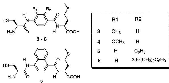
Figure 2. Structures of peptidomimetics with improved hydrophobic spacer.
