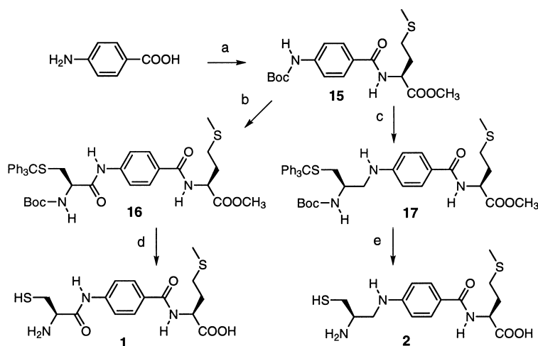
Scheme 1. Replacement of dipeptide in CVIM with 4-aminobenzoic acid. Reagents: (a) (1) (\text{Boc})_2\text{O} , NaOH, (2) (L)-methionine methyl ester; (b) (1) gaseous HCl in methanol, (2) N -Boc- S -trityl-(L)-cysteine, isobutyl chloroformate, \text{Et}_3\text{N} ; (c) (1) gaseous HCl in methanol, (2) N -Boc- S -trityl-(L)-cysteinyl, NaB(CN) \text{H}_3 ; (d) (1) aqueous LiOH, THF, (2) gaseous HCl in ether; (e) (1) aqueous LiOH, THF, (2) TFA, \text{Et}_3\text{SiH} .
