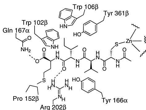
Figure 1. Active site contacts to the CAAX substrate for FTase. 26,27
